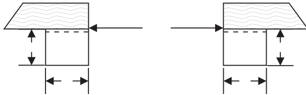
SQUARE PADS
